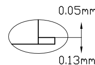
COPLANARITY
