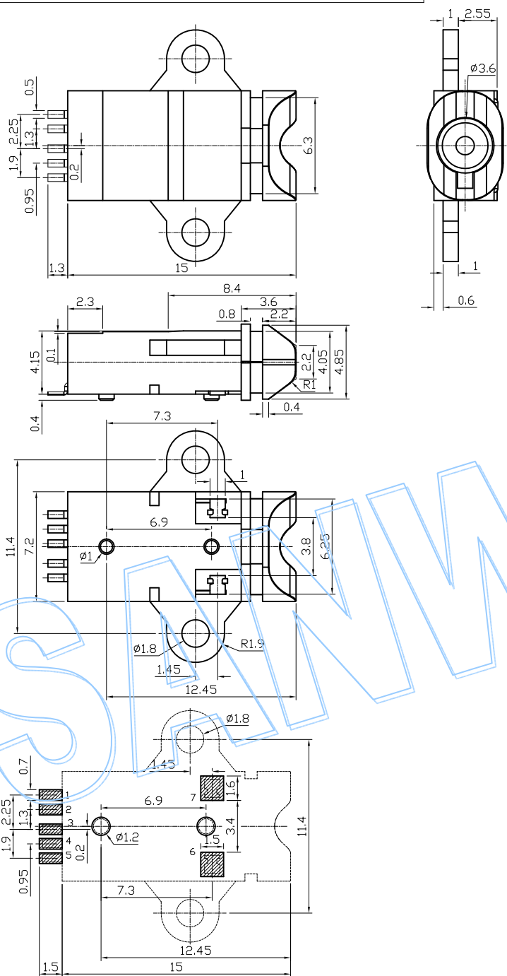
Recommended PAD Layout \Phi \pm 0.05 TOP VIEW
