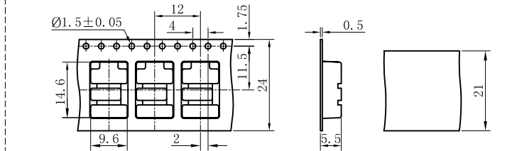
CARRIER TAPE
