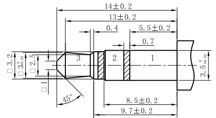
MATE PLUG
