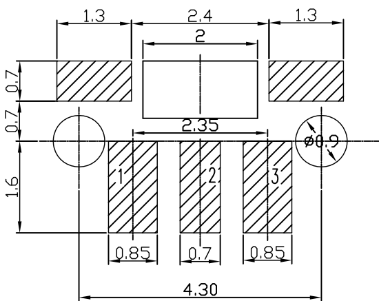
Recommended PAD Layout \Phi \pm 0.05 TOP VIEW
