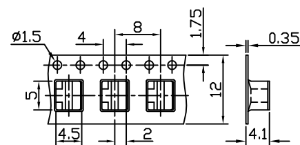
CARRIER TAPE
