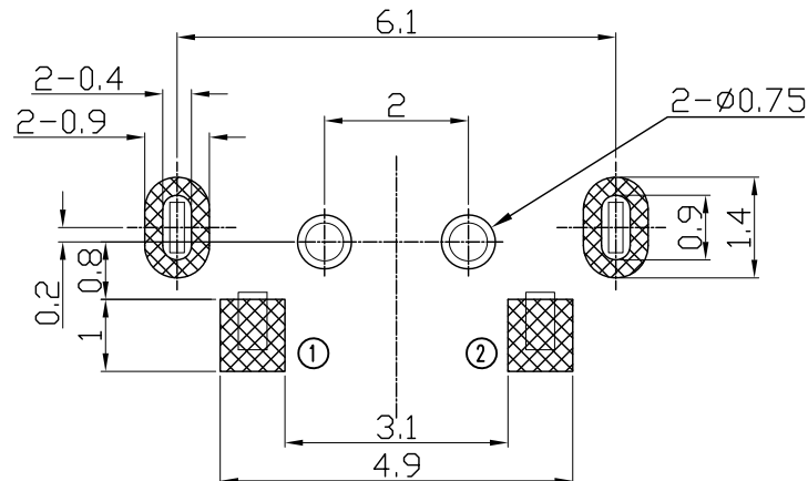
Recommended PAD Layout \pm 0.05 TOP VIEW
