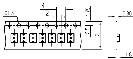
CARRIER TAPE
