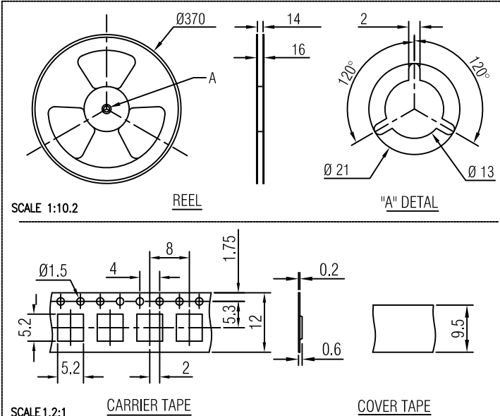
PACKING DETAIL <QTY:5000PCS/REEL>
