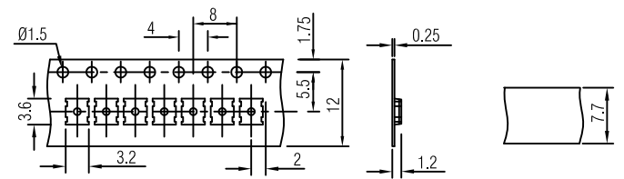
CARRIER TAPE
