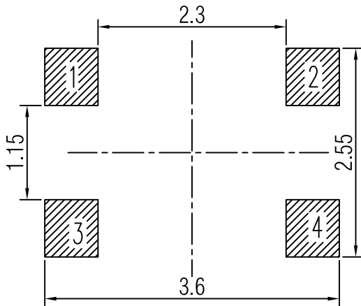
Recommended PAD Layout \pm 0.05 TOP VIEW
